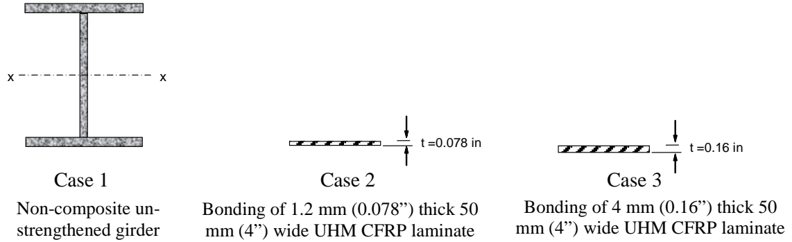
Fig. B1: Non-Composite Bridge Girder Types
