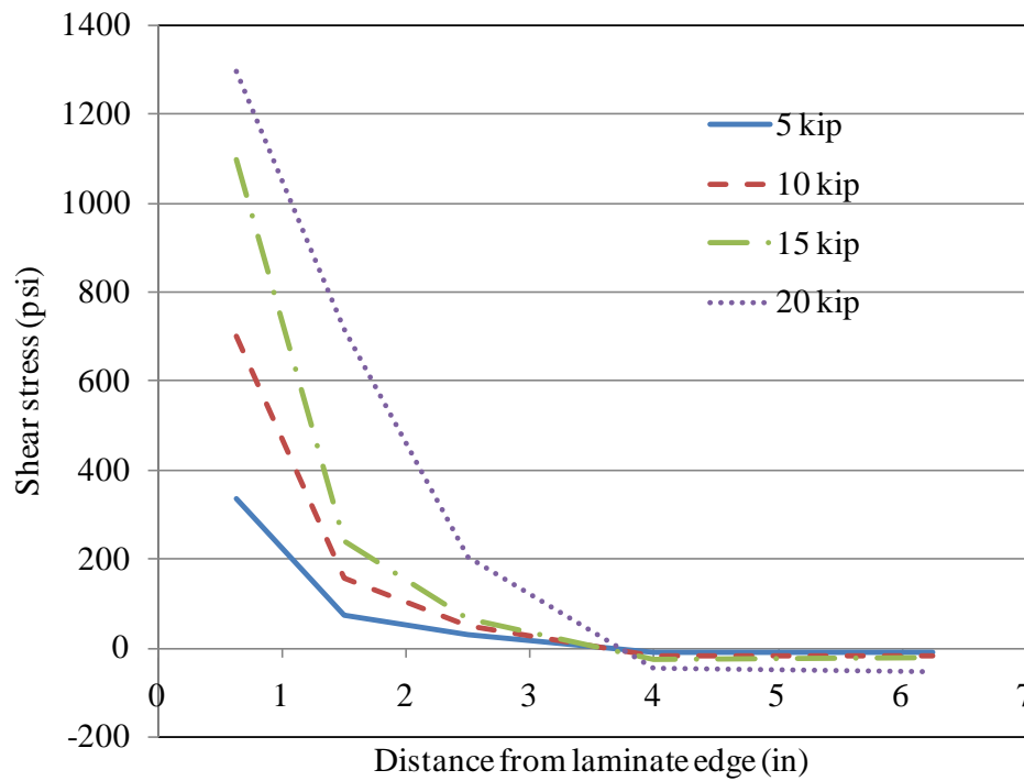
Fig. A22: Shear stress variation along laminate
