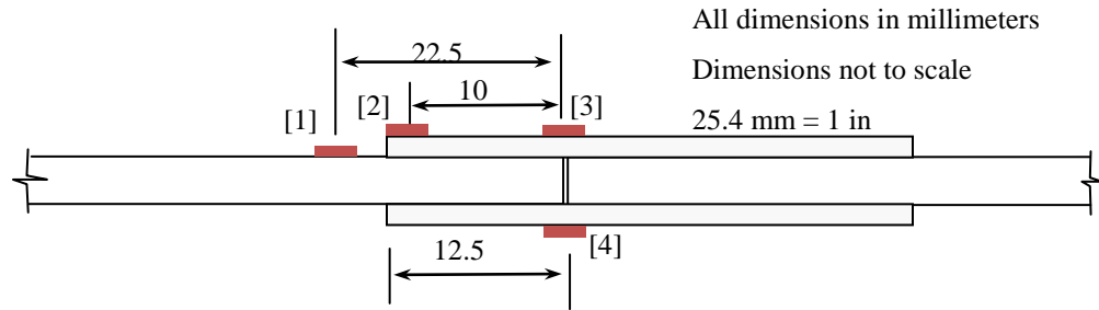
(a) 12.5 mm (0.5 in) Specimen
