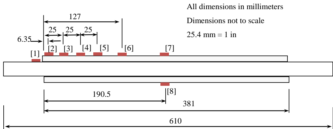
Fig. 2.24: Doubly Reinforced Steel Plate Specimen Gage Layout
